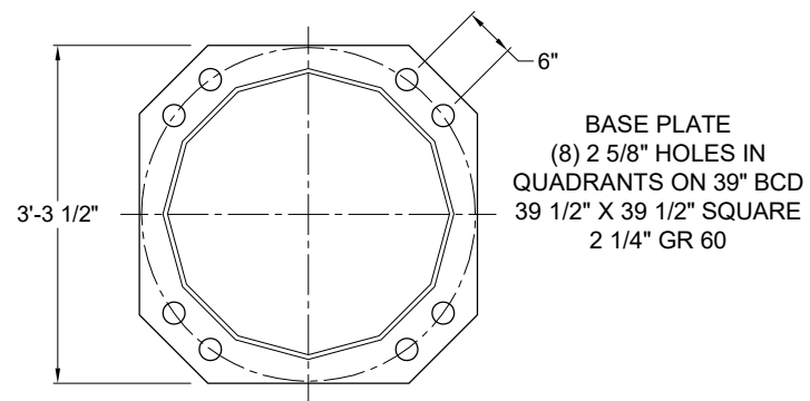
SECTION C-C BASE PLATE
