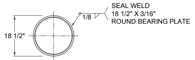
SECTION C-C BEARING PLATE
