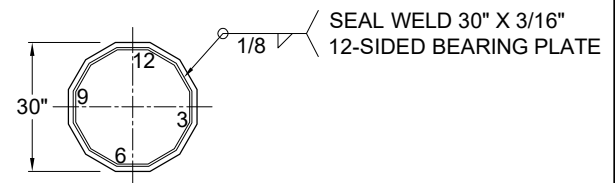
SECTION C-C BEARING PLATE
