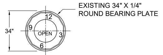
SECTION C-C BEARING PLATE
