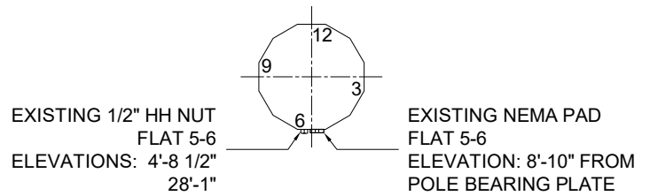
SECTION B-B GROUNDING
