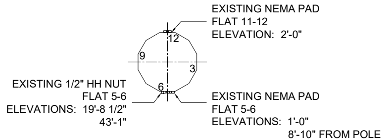
SECTION B-B GROUNDING
