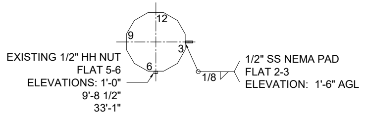
SECTION B-B GROUNDING
