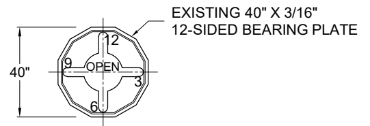
SECTION C-C BEARING PLATE
