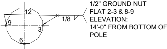
SECTION B-B GROUNDING
